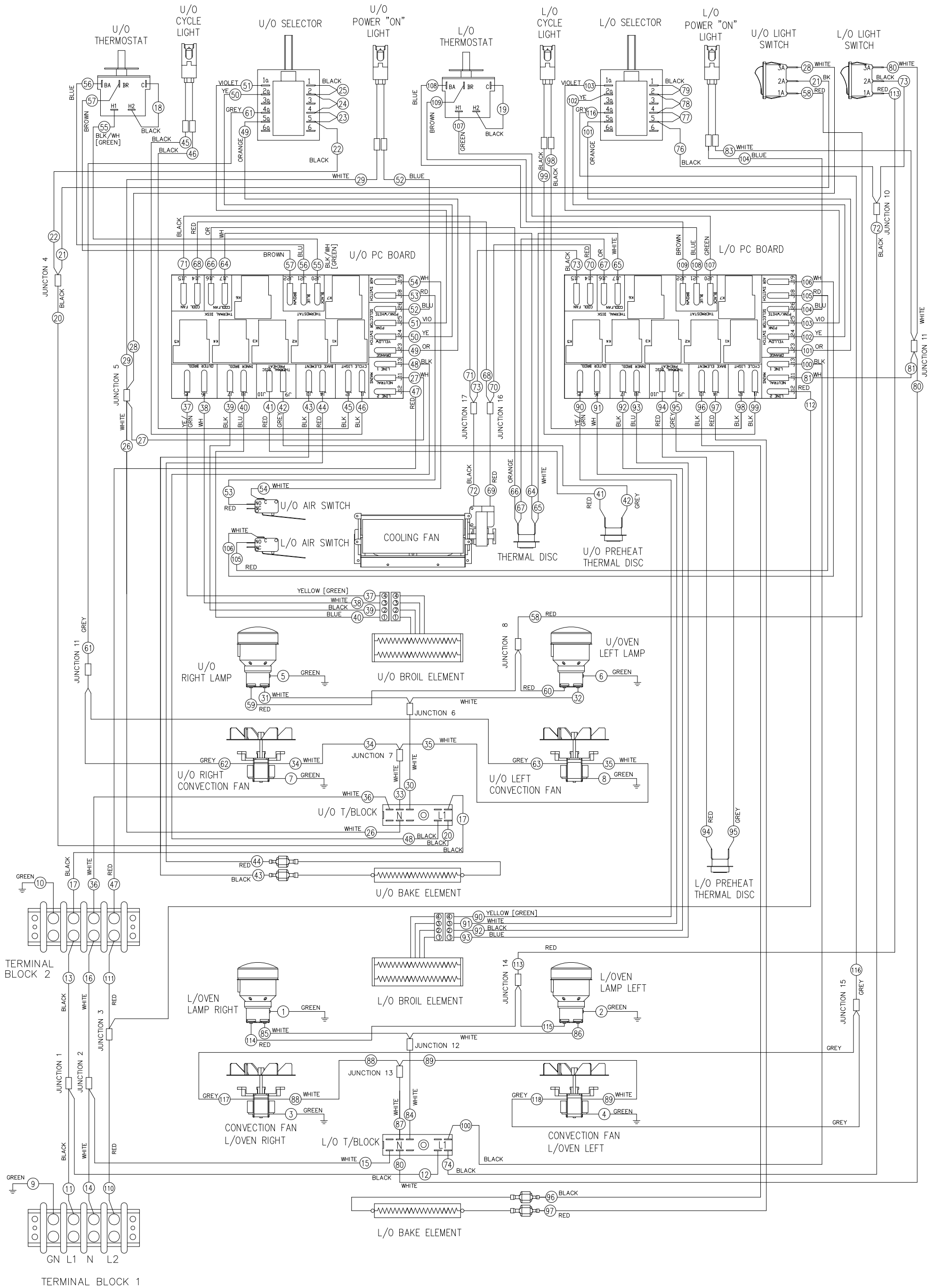
WIRING DIAGRAM [W/PC BOARD] REV. D DOUBLE ELECTRIC WALL OVEN MODELS AROFSE-230; AROFFE-230; AROSSE-230
