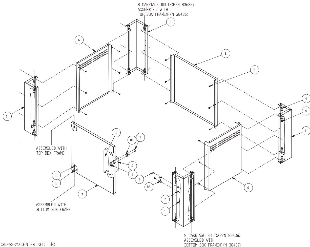
OGC30-ASSY.(CENTER SECTION)
