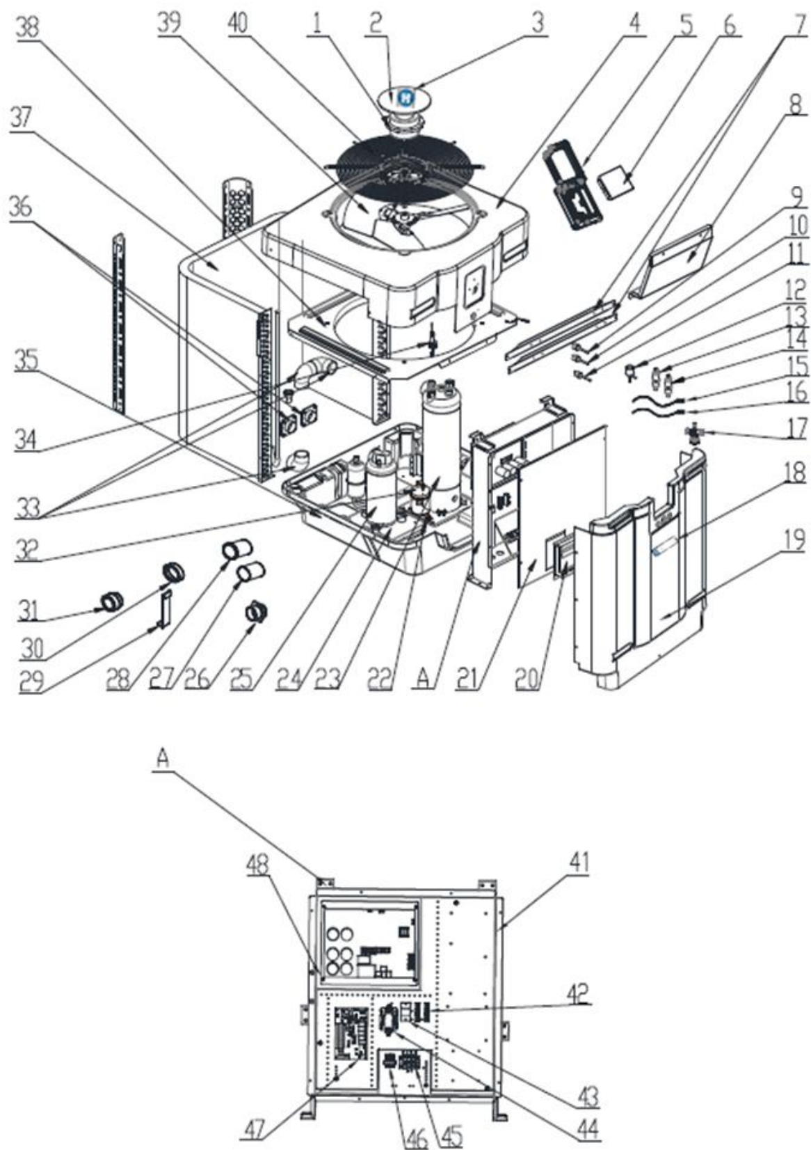
Figure16: Service Parts Exploded View
