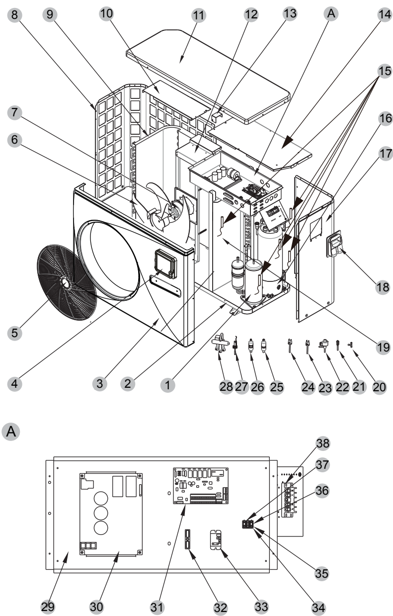
6.3 Exploded View - HP50AEE (1) Complete machine structure explosion diagram
