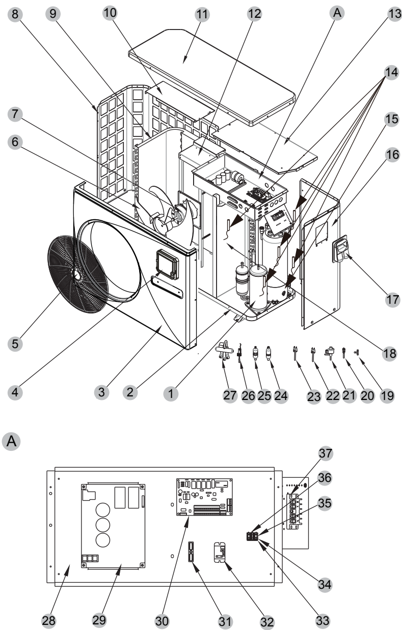
6.3 Exploded View - HP70AEE (1) Complete machine structure explosion diagram
