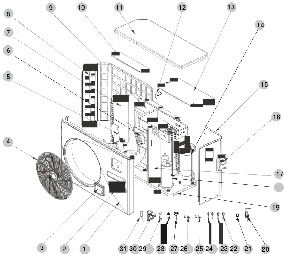
(1) Complete machine structure explosion diagram
