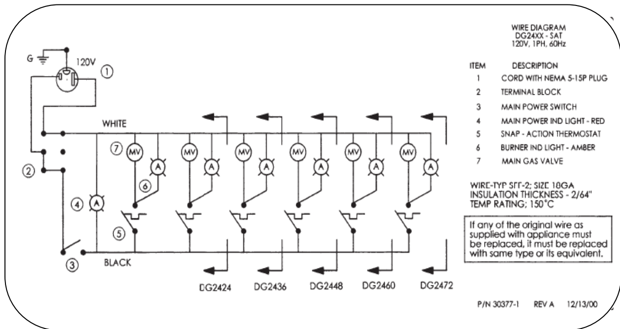
Griddles with standard snap-action thermostat.
