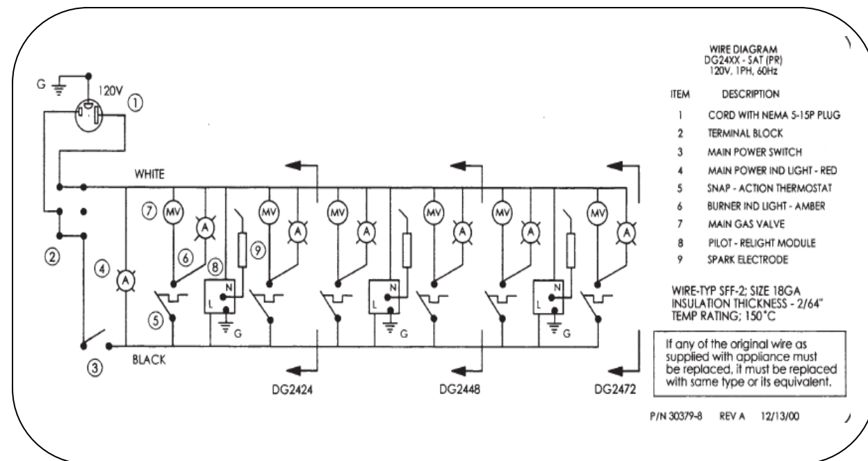
Griddles with snap-action T/stat and pilot relight option.
