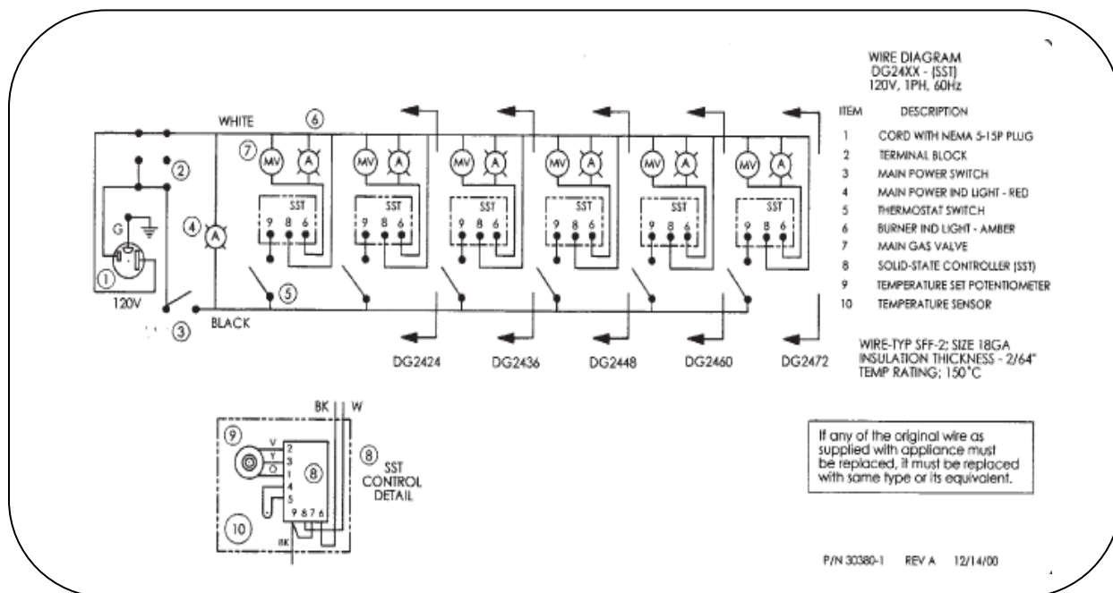
Griddles with solid-state T/stat.
